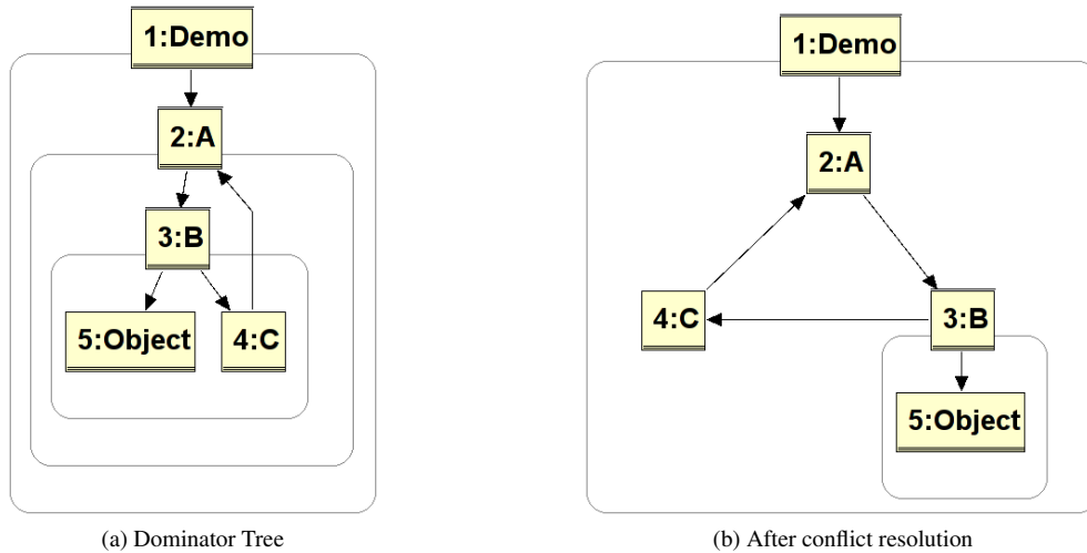
Figure 3: Contexts are depicted by rounded rectangles. Owner objects sit atop the context of objects they own.
